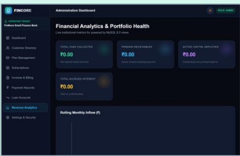
Administration Dashboard
